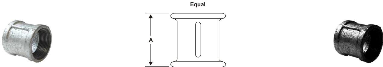
Fig 220 Socket
